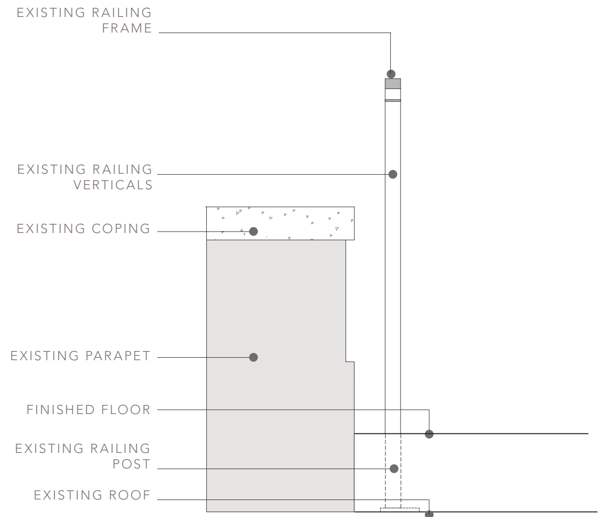
15TH FLOOR, PHW TERRACE - RAILING SECTION
