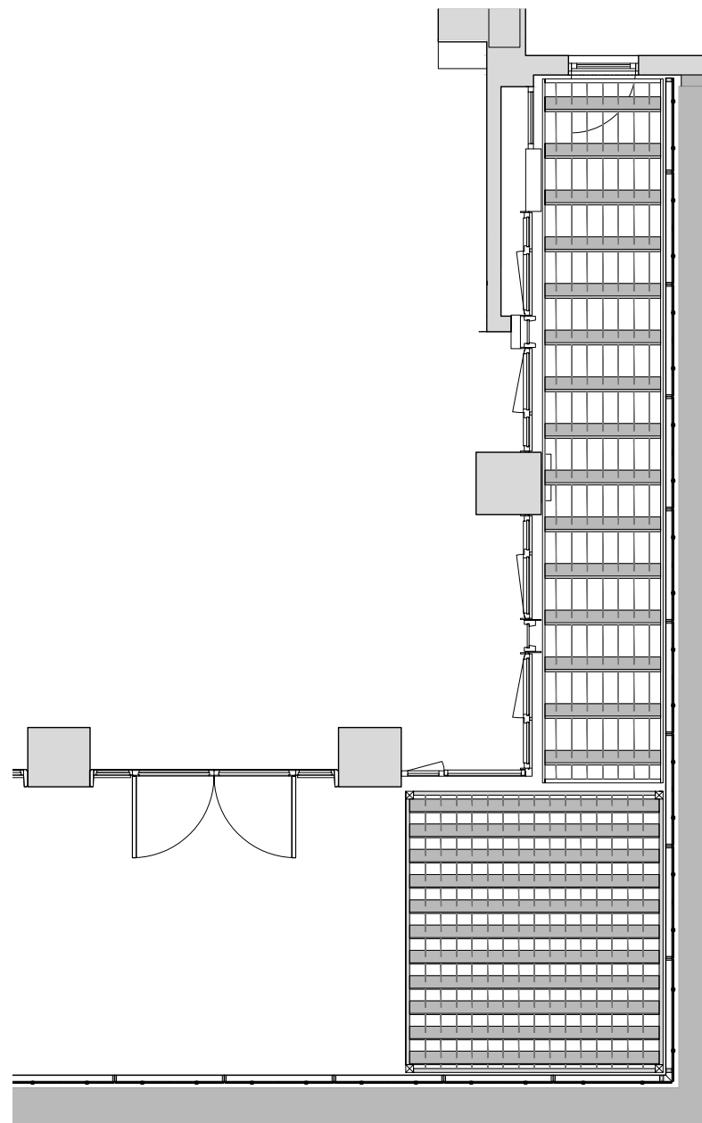
15TH FLOOR, PHW TERRACE - TRELLIS PLAN
