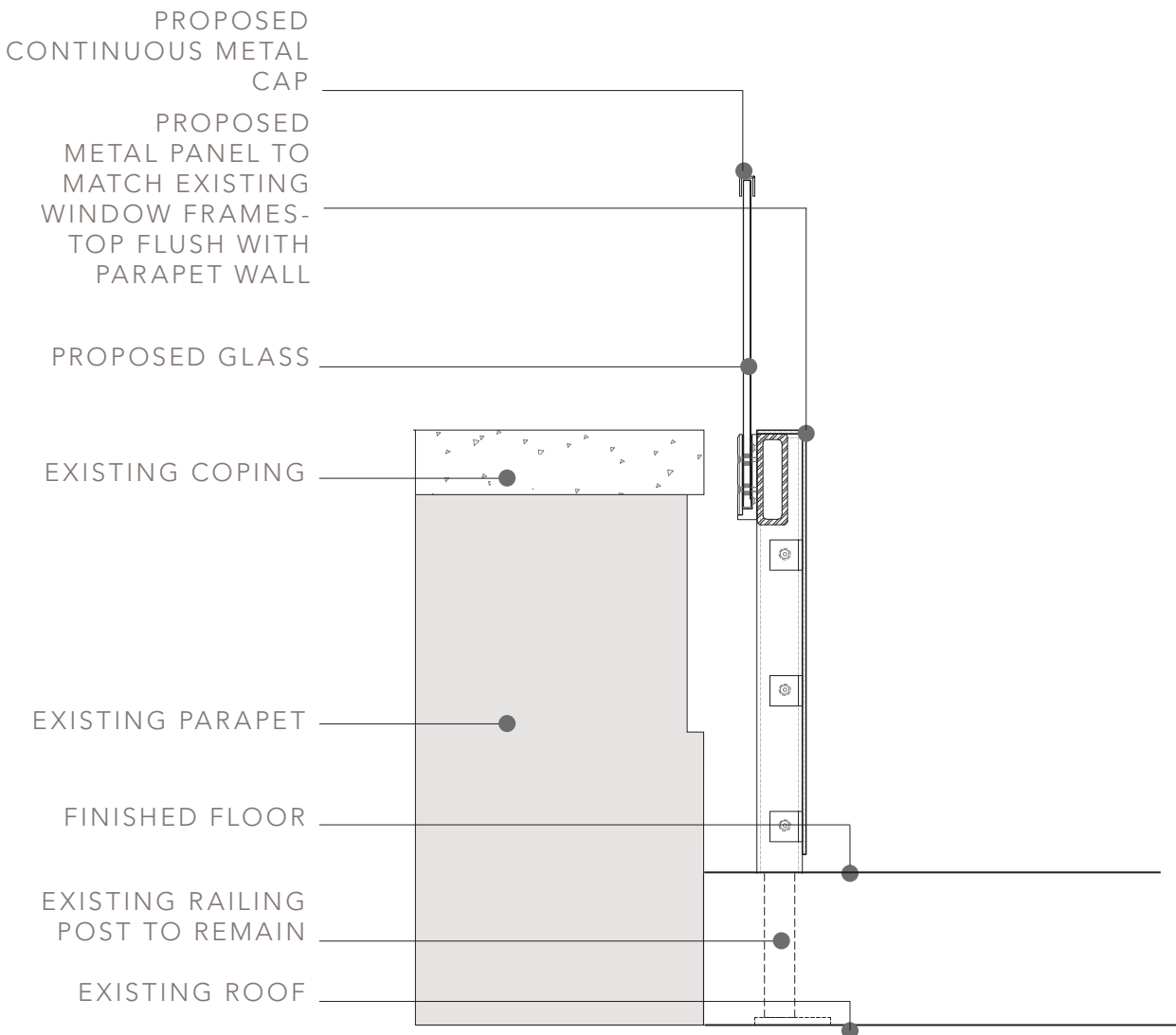
15TH FLOOR, PHW TERRACE - RAILING SECTION
