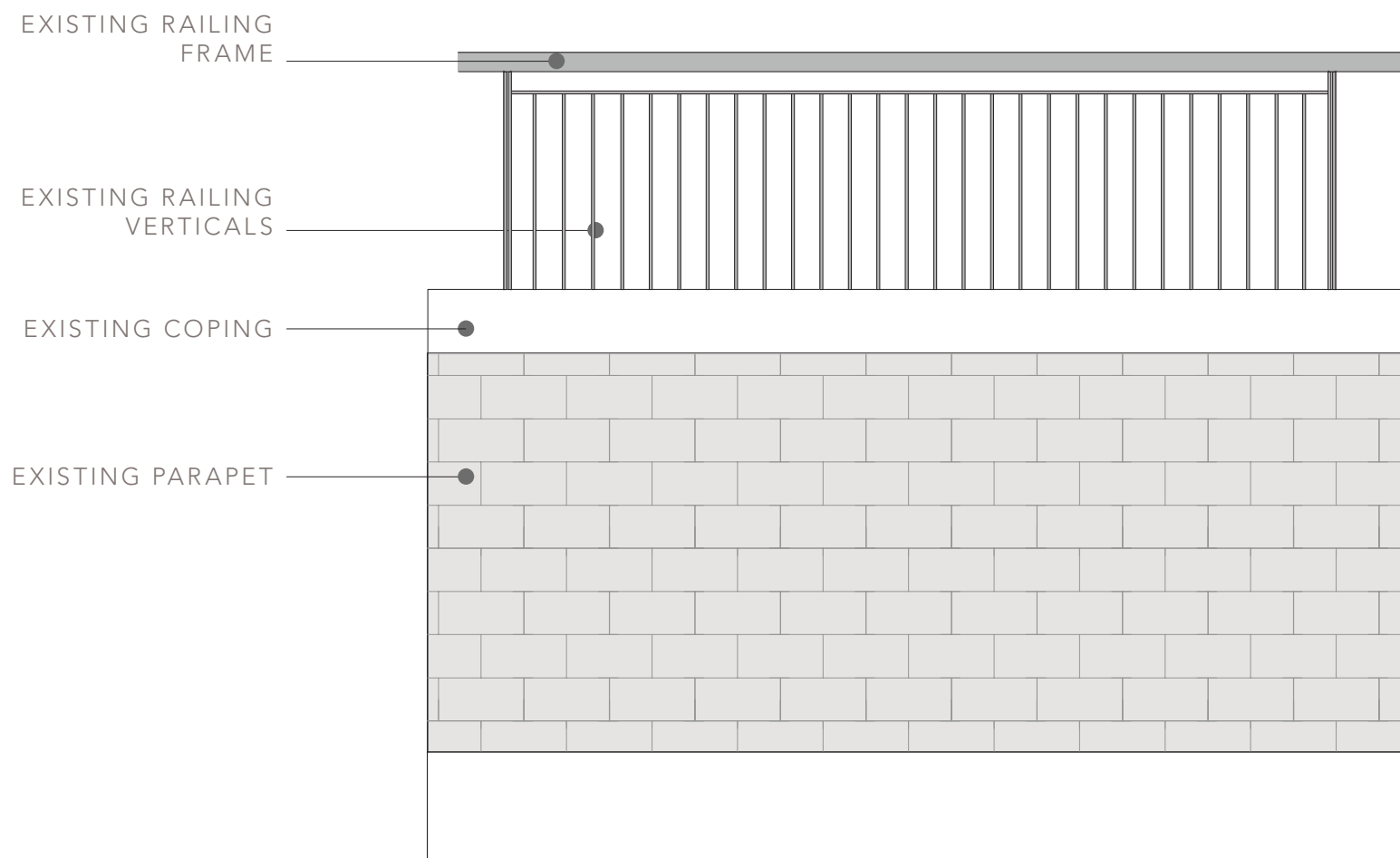
15TH FLOOR, PHW TERRACE - RAILING ELEVATION
